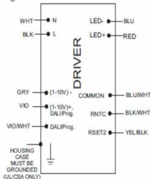
Wire Diagram
